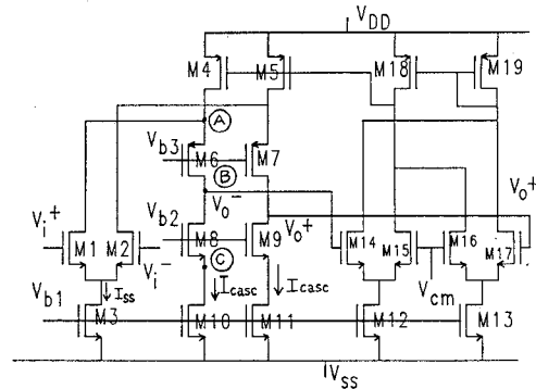
Fig. 1. Fully differential folded-cascode amplifier (after [4]).
